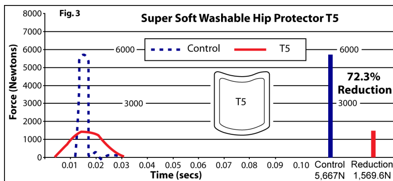
Fig 3. Force plotted against time for the control & supersoft washable hip protector, Item 179SSWT5.
