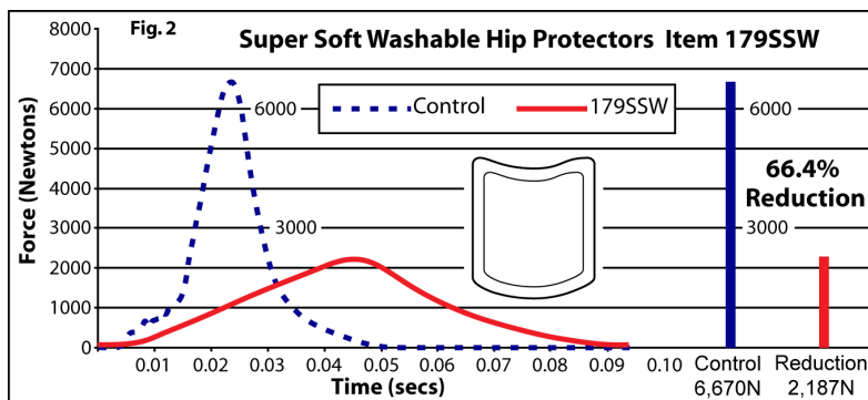
Fig 2. Force plotted against time for the control & supersoft washable hip protector, Item 179SSW.
