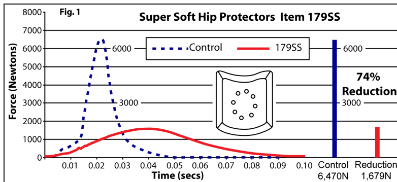
Fig 1. Force plotted against time for the control and 179SS hip protector.
